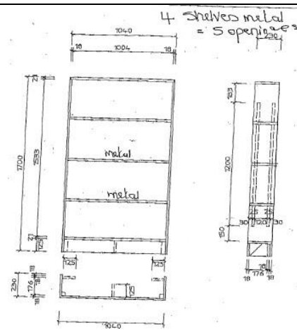
FIG 14 (a) WALL SHELF
